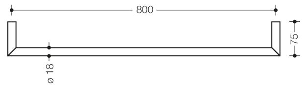
Abmessungen in mm
