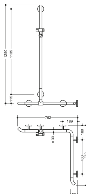
Abmessungen in mm
