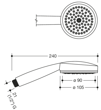
Abmessungen in mm
