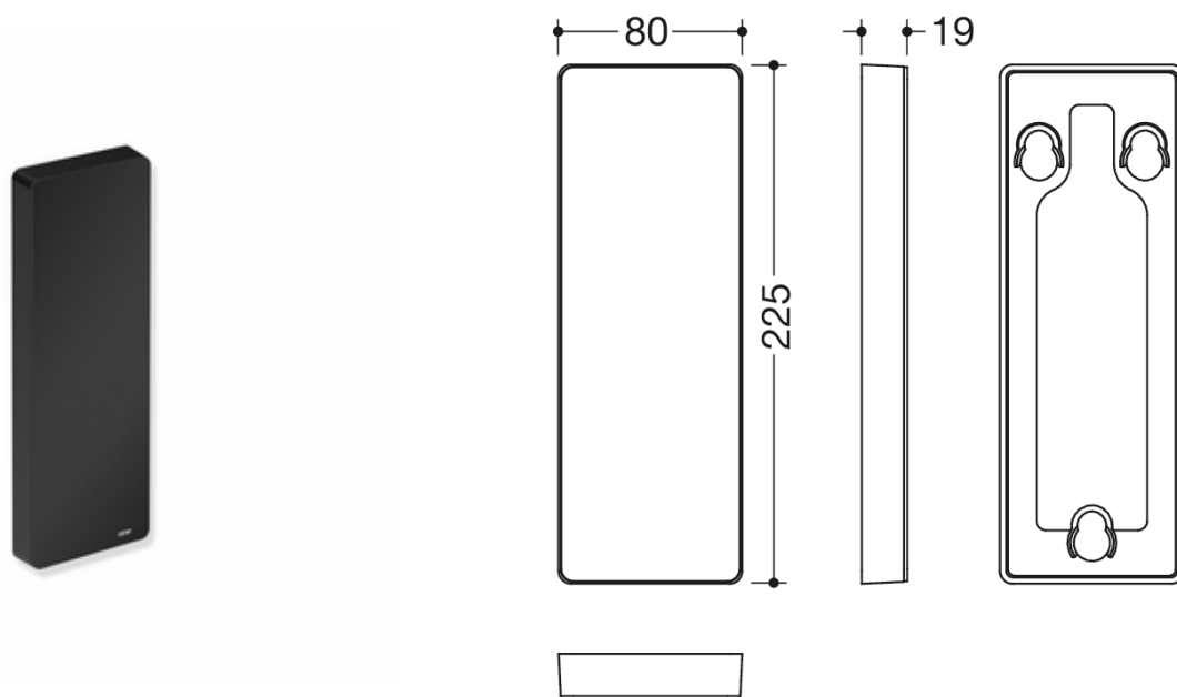
Abmessungen in mm
