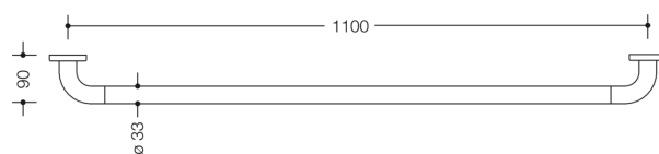
Abmessungen in mm
