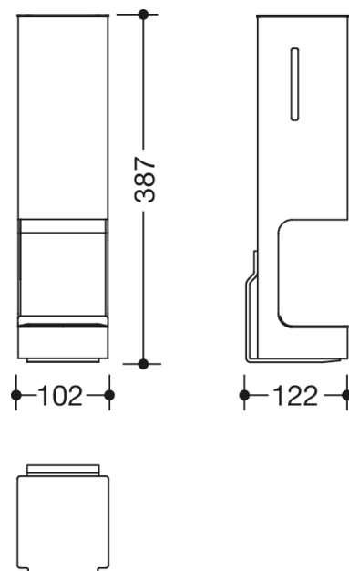
Abmessungen in mm
