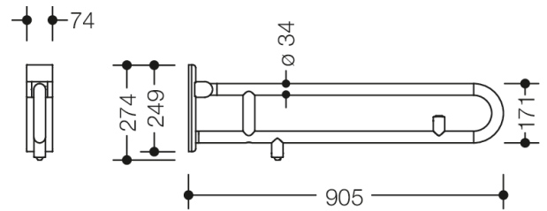
Abmessungen in mm
