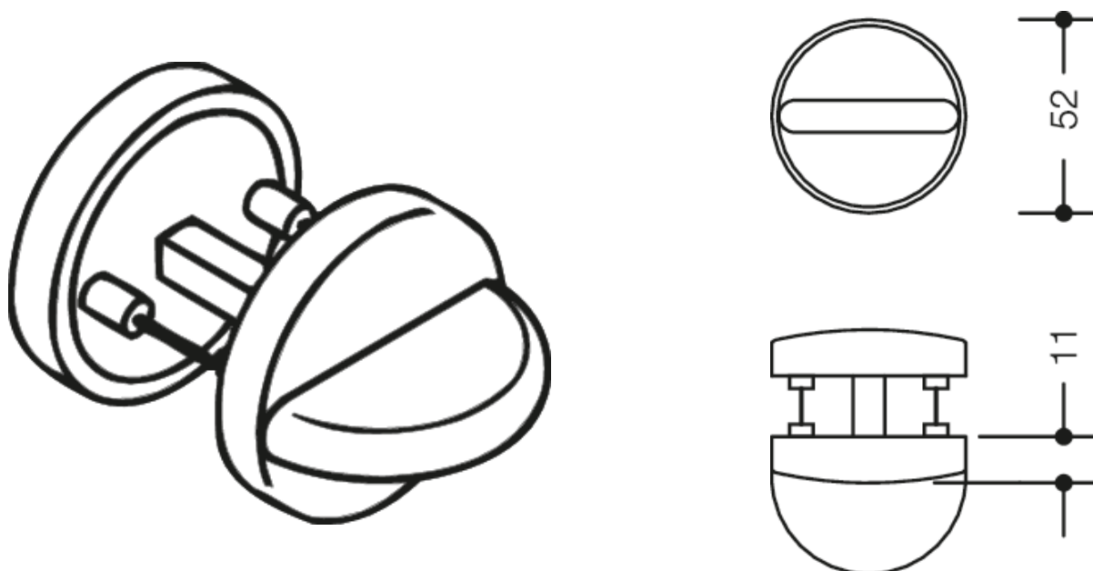
Abmessungen in mm
