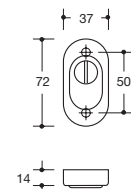
Security escutcheon with cylinder cover 316...Z
